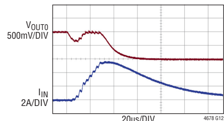
Single Phase Single Output Short-Circuit Protection, No Load
