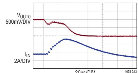
Single Phase Single Output Short-Circuit Protection, 18A Load
