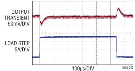
Single Channel Load Transient Response 50% to 100% Load Step, 12A/ \mu\text{s} 12V IN to 1.5V OUT
