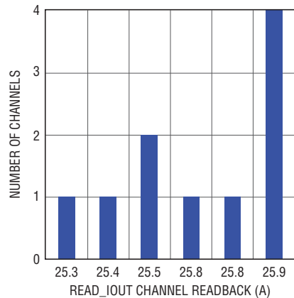
READ_IOUT of 10 LTM4678 Channels 12\text{V}_{\text{IN}} , 1\text{V}_{\text{OUT}} , T_J = 25^{\circ}\text{C} , I_{\text{OUT}n} = 25\text{A} , System Having Reached Thermally Steady-State Condition, No Airflow
