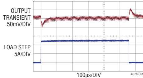
Single Channel Load Transient Response 50% to 100% Load Step, 12A/ \mu\text{s} 12V IN to 0.9V OUT
