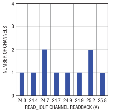
READ_IOUT of 10 LTM4678 Channels 12\text{V}_{\text{IN}} , 1\text{V}_{\text{OUT}} , T_J = 125^{\circ}\text{C} , I_{\text{OUT}n} = 25\text{A} , System Having Reached Thermally Steady-State Condition, No Airflow
