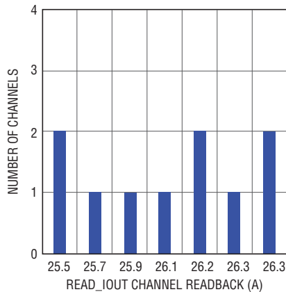
READ_IOUT of 10 LTM4678 Channels 12\text{V}_{\text{IN}} , 1\text{V}_{\text{OUT}} , T_J = -40^{\circ}\text{C} , I_{\text{OUT}n} = 25\text{A} , System Having Reached Thermally Steady-State Condition, No Airflow
