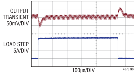
Single Channel Load Transient Response 50% to 100% Load Step, 12A/ \mu\text{s} 12V IN to 1.2V OUT
