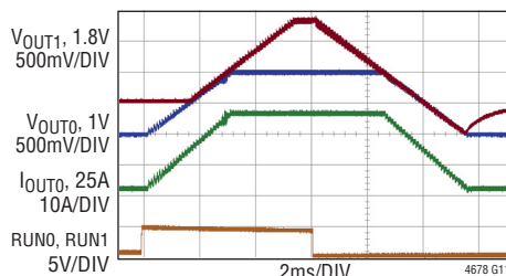
Dual Output Concurrent Rail, Start-Up/Shut Down, Pre-Bias
