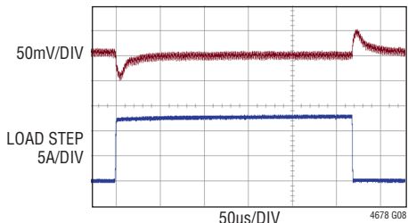
Single Channel Load Transient Response 50% to 100% Load Step, 12A/ \mu\text{s} 12V IN to 1.8V OUT
