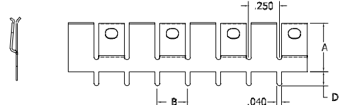
FIGURE 6 .25" Pin Spacing, With Standoff
