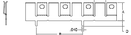
FIGURE 4 1.0" Pin Spacing, With Standoff
