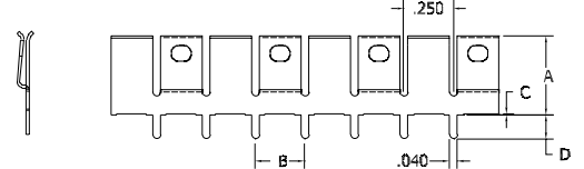
FIGURE 6 .25" Pin Spacing, With Standoff
