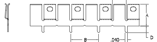
FIGURE 3 1.0" Pin Spacing, No Standoff
