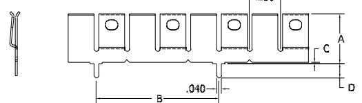
FIGURE 5 .25" Pin Spacing, No Standoff
