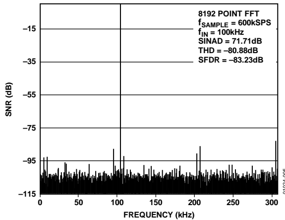
Figure 5. AD7476 Dynamic Performance at 600 kSPS
