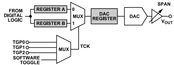
Figure 53. Toggle Operation
