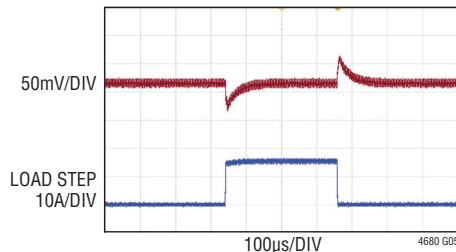
FIGURE 46 CIRCUIT, 12V TO 0.9V, FREQ = 250kHz C_{\text{OUT}} = 470\mu\text{F} \times 3 POSCAP, 100\mu\text{F} \times 4 CERAMIC R_{\text{COMP}} = 17\text{k} , EA-GM = 3.69ms, \text{COMP}_{\text{Pa}} = 3.3\text{nF} , \text{COMP}_{\text{Pb}} = 68\text{pF} I_{\text{LIM}} LOW, V_{\text{OUT}} RANGE LOW
