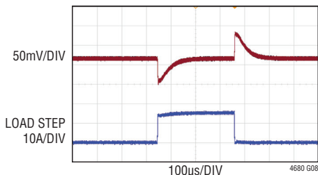
FIGURE 46 CIRCUIT, 12V TO 2.5V, FREQ = 575kHz C_{\text{OUT}} = 470\mu\text{F} \times 2 POSCAP, 100\mu\text{F} \times 4 CERAMIC R_{\text{COMP}} = 20\text{k} , EA-GM = 1.68ms, \text{COMP}_{\text{Pa}} = 3.3\text{nF} , \text{COMP}_{\text{Pb}} = 68\text{pF} I_{\text{LIM}} LOW, V_{\text{OUT}} RANGE LOW
