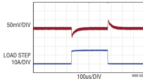
FIGURE 46 CIRCUIT, 12V TO 1.2V, FREQ = 350kHz C_{\text{OUT}} = 470\mu\text{F} \times 2 POSCAP, 100\mu\text{F} \times 4 CERAMIC R_{\text{COMP}} = 17\text{k} , EA-GM = 3.69ms, \text{COMP}_{\text{Pa}} = 3.3\text{nF} , \text{COMP}_{\text{Pb}} = 68\text{pF} I_{\text{LIM}} LOW, V_{\text{OUT}} RANGE LOW
