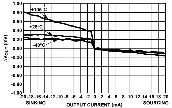
FIGURE 107. LOAD REGULATION OVER-TEMPERATURE
