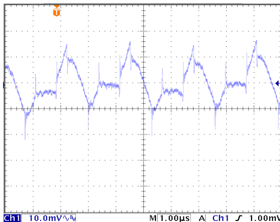
Output Ripple & Noise (VIN = 12 V, IOUT = 20 A, COUT = 10µF || 1µF, scope = 20 MHz BW) Vertical = 10 mV/div., Sweep = 1µS/div.
