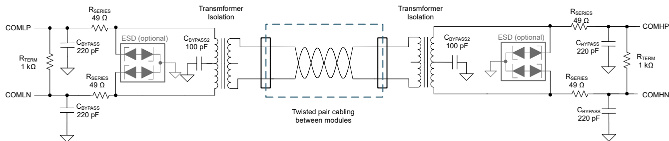
Figure 9-15. Transformer Isolation
