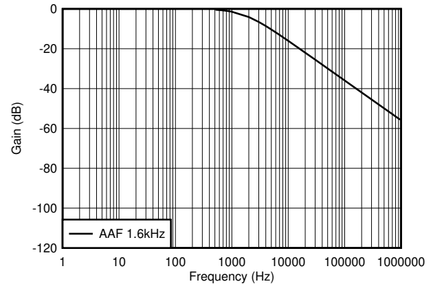
Figure 7-4. MAIN ADC Filter
