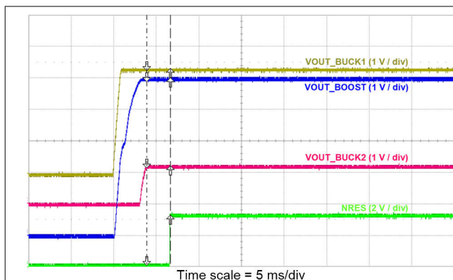
Figure 12-44. Start-up Showing NRES Output With Short NRES Extension Delay
