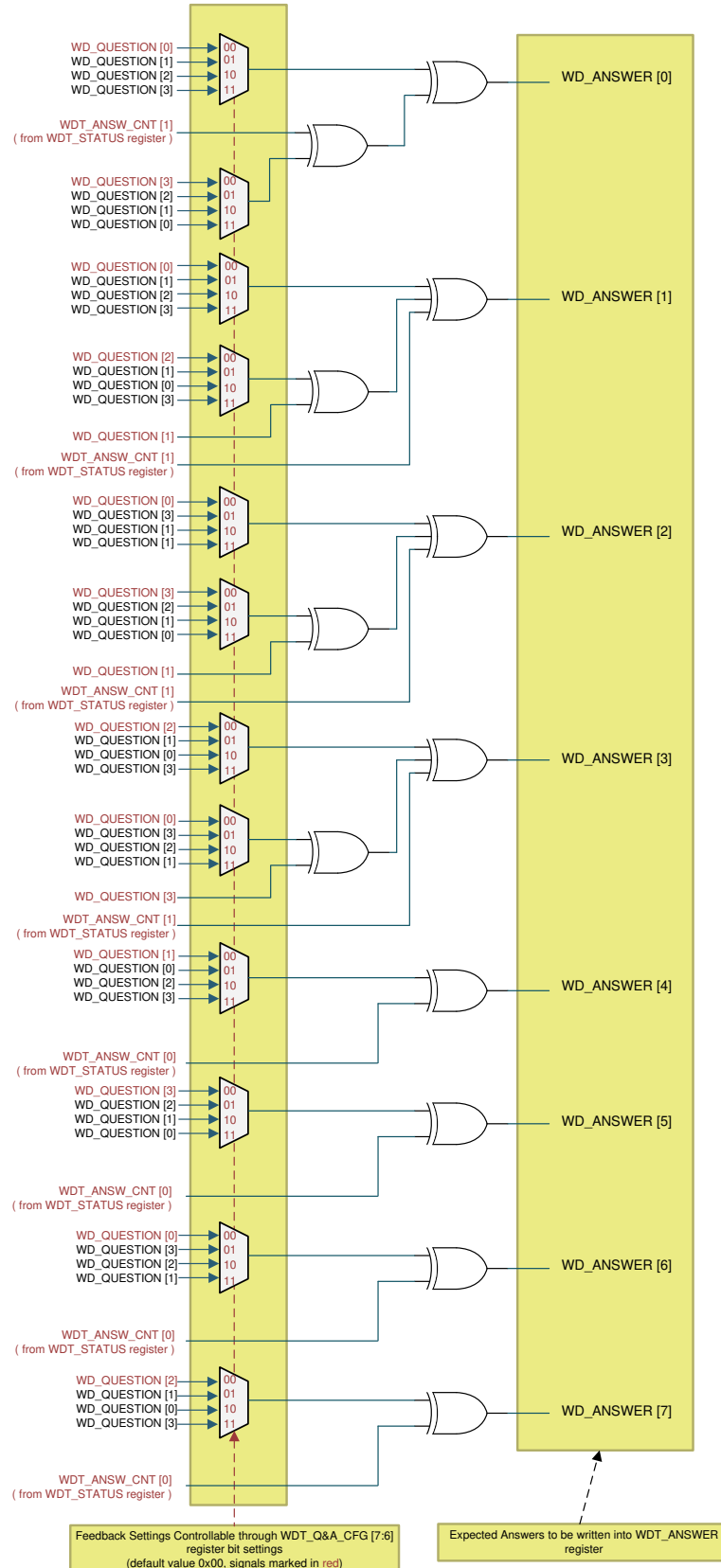
Figure 11-19. WD Expected Answer Generation
