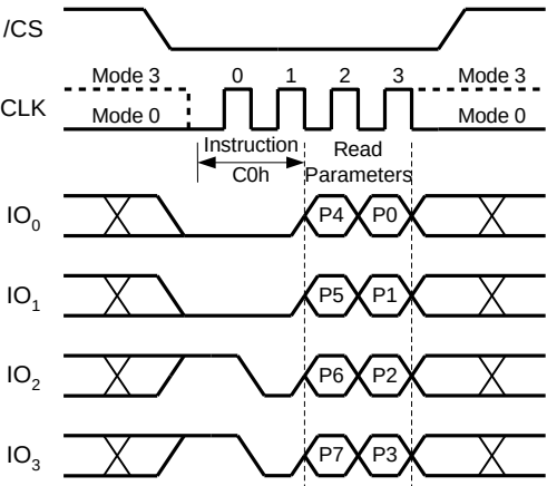
Figure 31. Set Read Parameters Instruction (QPI Mode only)
