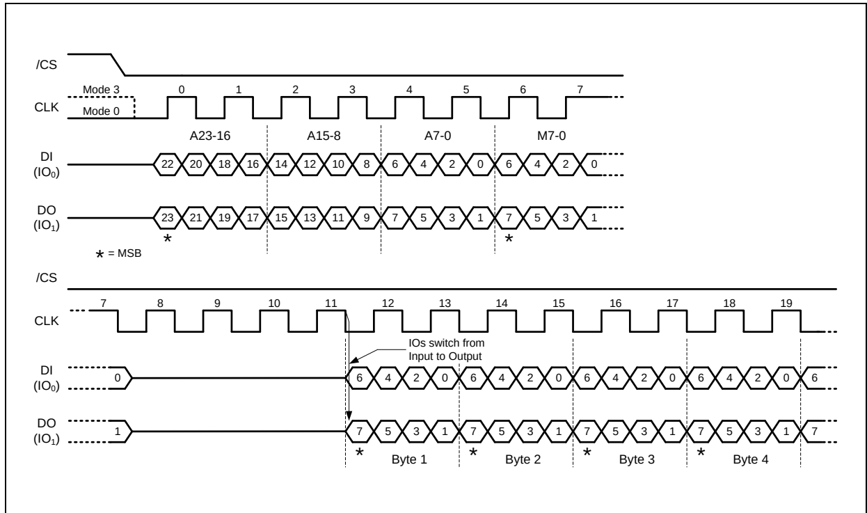
Figure 24b. DTR Fast Read Dual I/O (Previous instruction set M5-4=10, SPI Mode only)
