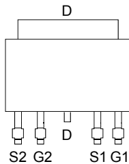
Pinout Top View
