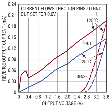
Reverse Output Current (0.6V)
