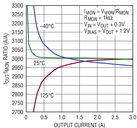
I_{OUT}/I_{MON} Ratio
