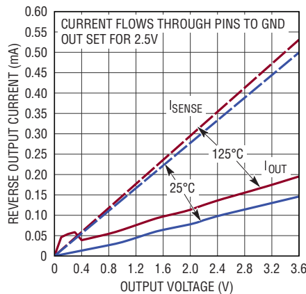
Reverse Output Current (2.5V)
