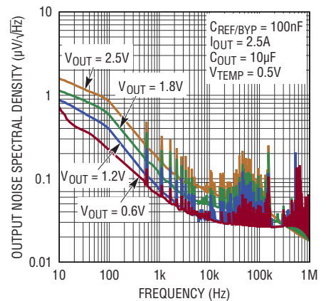
Output Noise Spectral Density vs V_{OUT}
