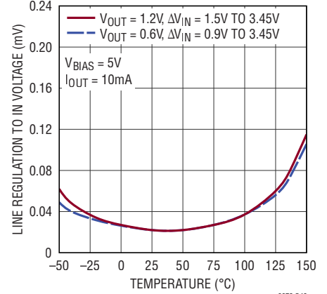
Line Regulation to V_{IN}
