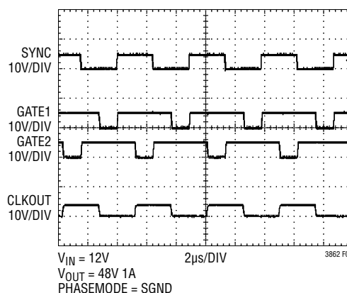
Figure 7. Synchronization of the LTC3862 to an External Clock Using the PLL
