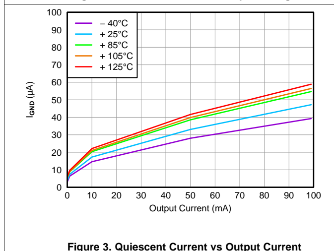
Figure 3. Quiescent Current vs Output Current
