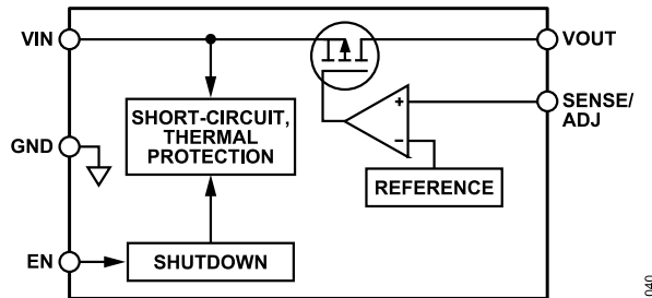
Figure 42. Internal Block Diagram
