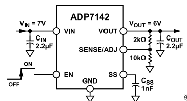
Figure 2. ADP7142 with 5 V Output Adjusted to 6 V
