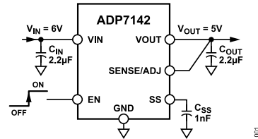
Figure 1. ADP7142 with Fixed Output Voltage, 5 V
