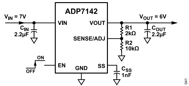
Figure 43. Typical Adjustable Output Voltage Application Schematic
