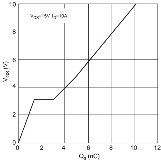
Fig. 11 Gate Charge
