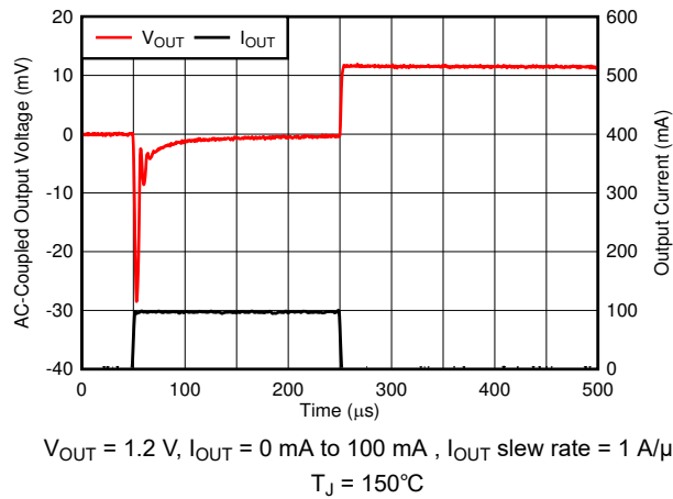
Figure 6-49. Load Transient
