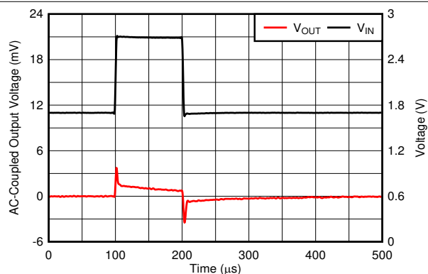
Figure 6-25. Line Transient
