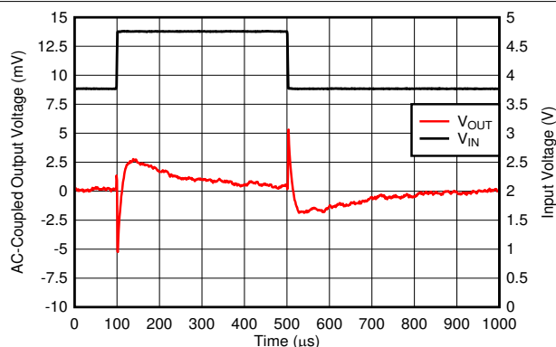
Figure 6-25. Line Transient
