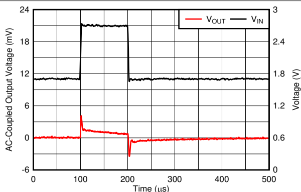
Figure 6-26. Line Transient
