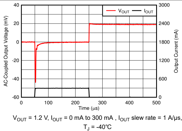
Figure 6-51. Load Transient
