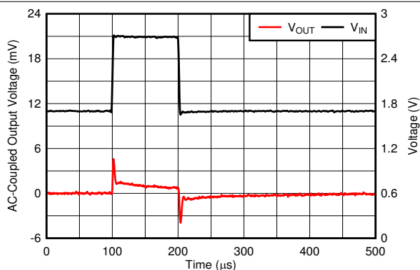
Figure 6-26. Line Transient
