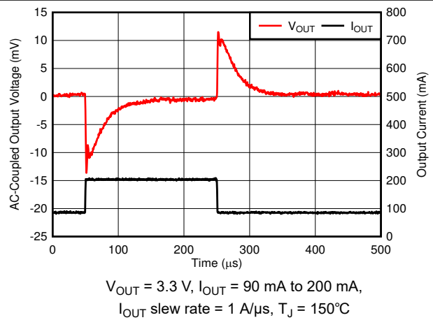
Figure 6-64. Load Transient
