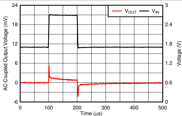
Figure 6-28. Line Transient
