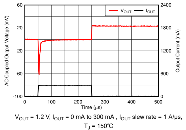
Figure 6-52. Load Transient
