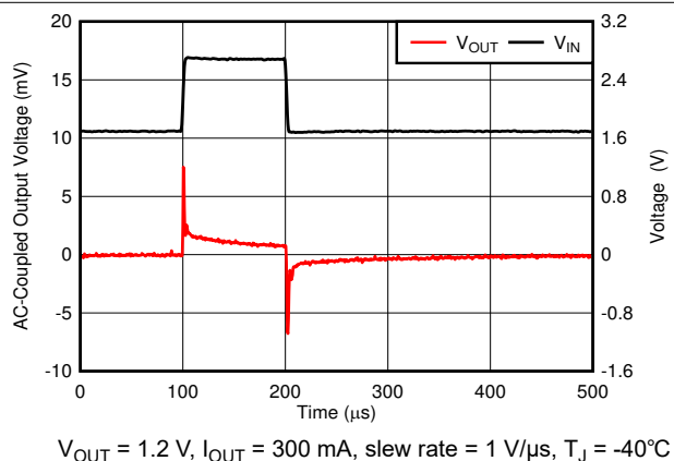
Figure 6-33. Line Transient
