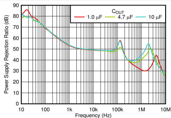
Figure 6-68. PSRR vs Frequency and C_{OUT}
