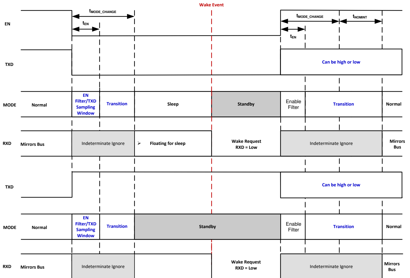
Figure 8-15. Mode Transitions
