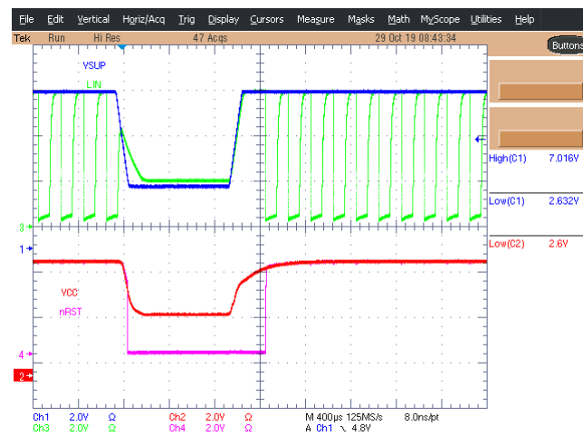
Figure 10-18. TLIN10285-Q1 Brownout
