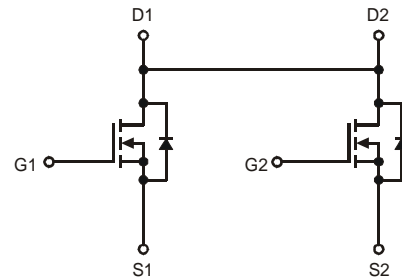
Equivalent Circuit
