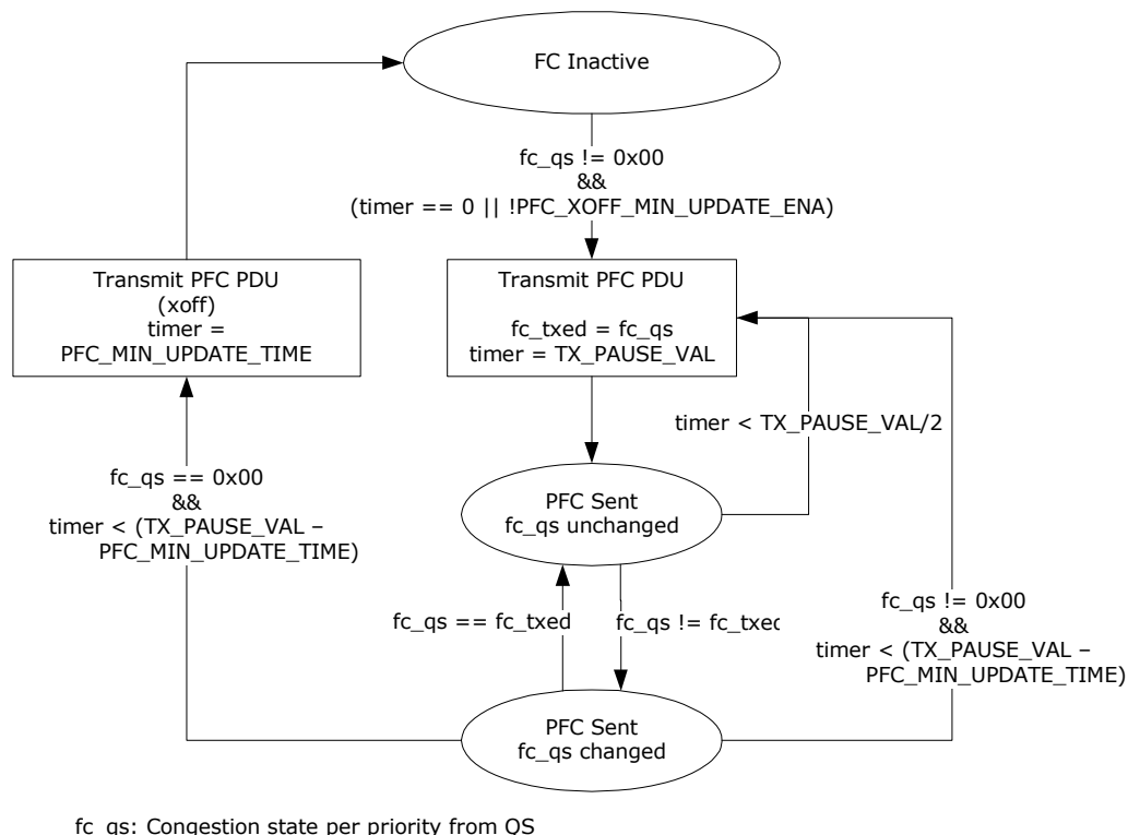
Figure 126 • PFC Generation per Port
