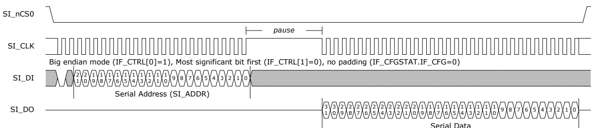
Figure 134 • Read Sequence for SI_CLK Pause
