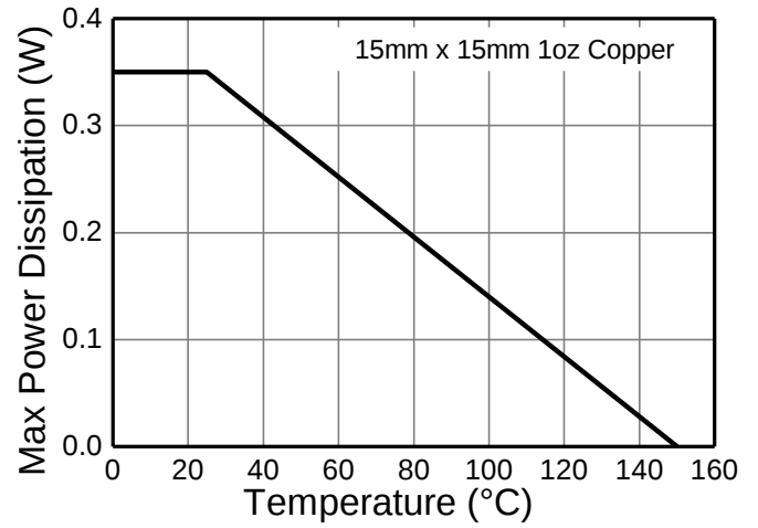
Figure 2. Derating Curve
