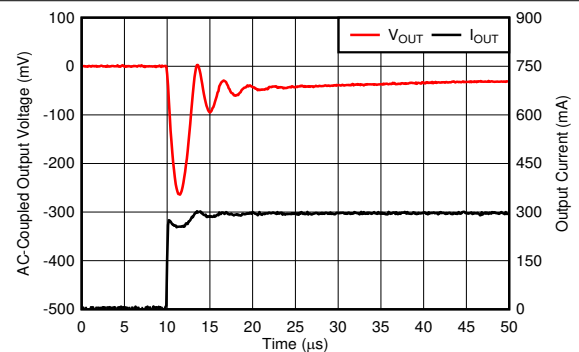
Figure 6-22. Load Transient
