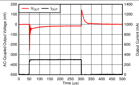
Figure 6-21. Load Transient
