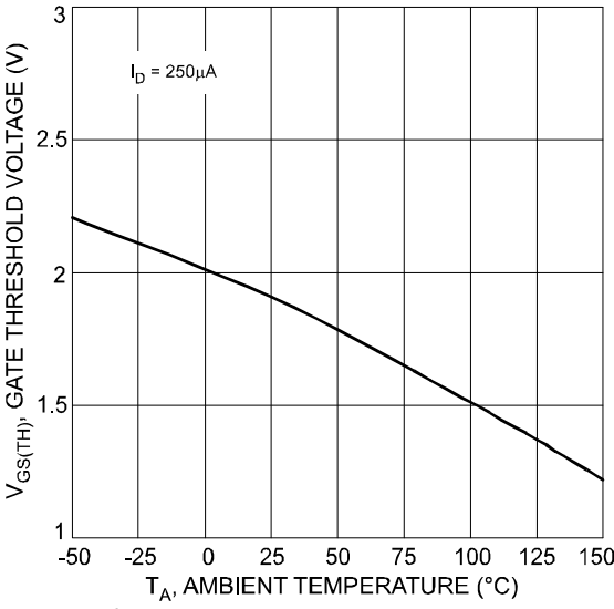
Fig. 5 Gate Threshold Voltage vs. Ambient Temperature
