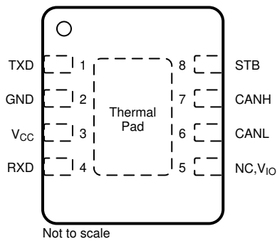
Figure 6-3. DRB Package, 8-Pin VSON, Top View
