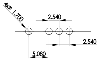
RECOMMENDED THROUGH HOLES FOR LAND PATTERN
