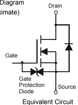
Equivalent Circuit
