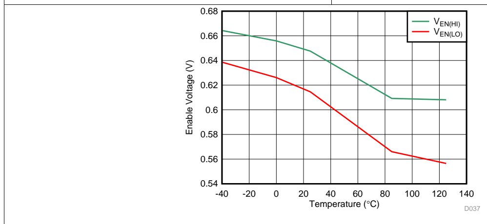
Figure 47. Enable High and Low Thresholds vs Temperature
