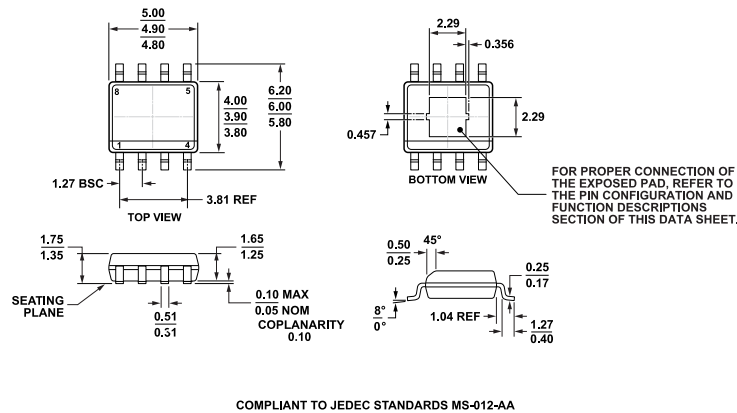
Figure 68. 8-Lead Standard Small Outline Package, with Exposed Pad [SOIC_N_EP] Narrow Body (RD-8-1) Dimensions shown in millimeters
