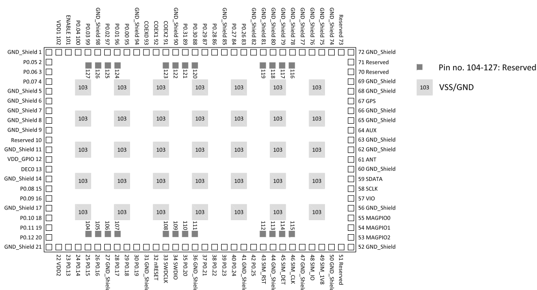
Figure 116: LGA pin assignments, top view
