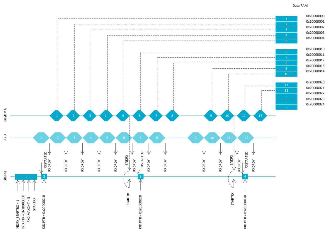
Figure 106: UARTE reception
