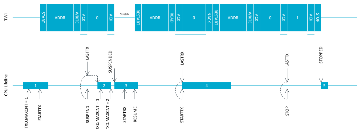
Figure 94: Double repeated start sequence
