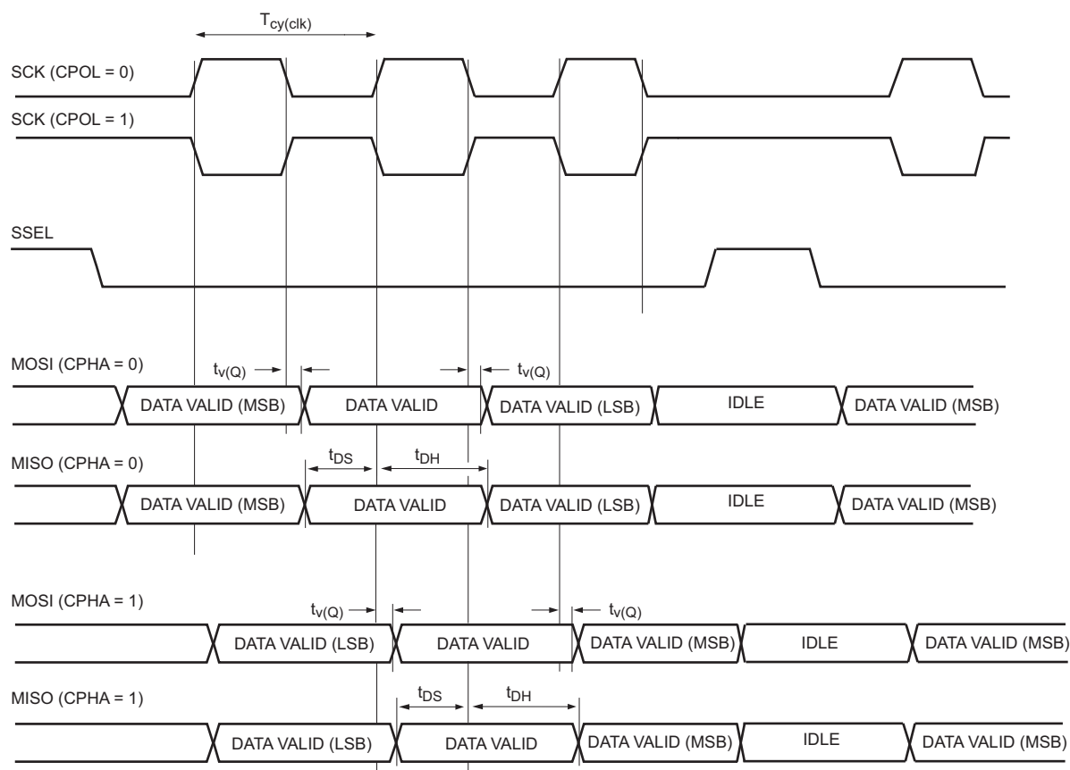
Fig 22. SPI master timing
