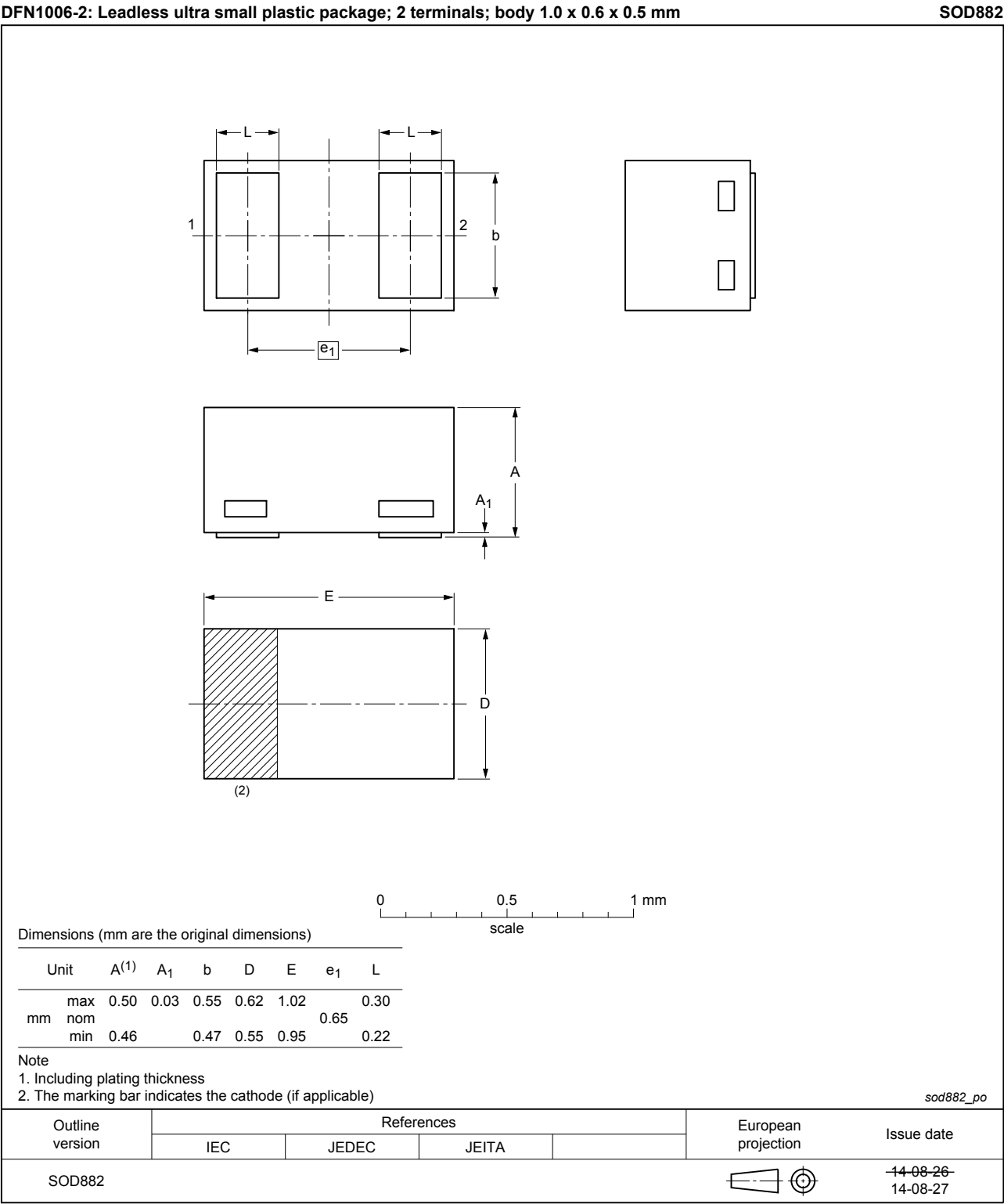
Fig. 12. Package outline DFN1006-2 (SOD882)
