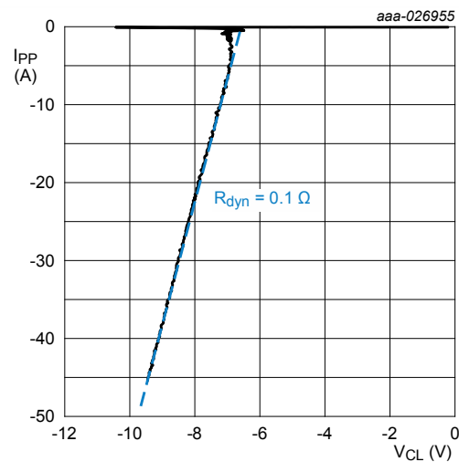
Fig. 6. Negative clamping voltage (TLP); typical values t_p = 100 \text{ ns}; \text{Transmission Line Pulse (TLP)}
