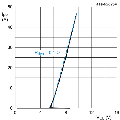
Fig. 5. Positive clamping voltage (TLP); typical values t_p = 100 \text{ ns}; \text{Transmission Line Pulse (TLP)}
