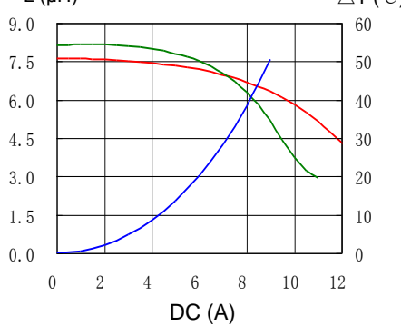
8. CDRH127L125NP-220MC
