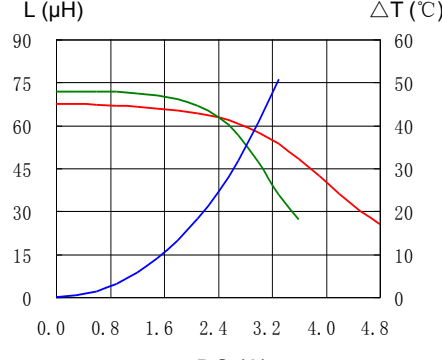
11. CDRH127L125NP-680MC
