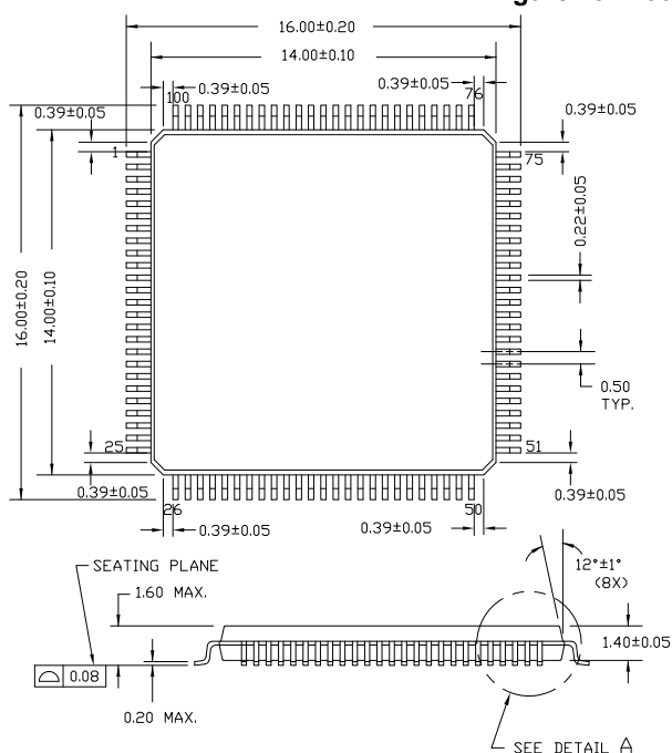
Figure 19. 100-TQFP 14.0 × 14.0 × 1.4 mm
