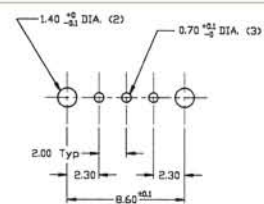
P.C. MOUNTING
