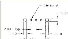
P.C. MOUNTING
