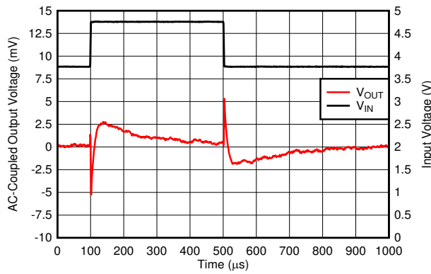
Figure 6-25. Line Transient
