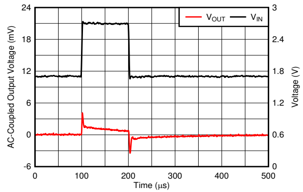
Figure 6-26. Line Transient
