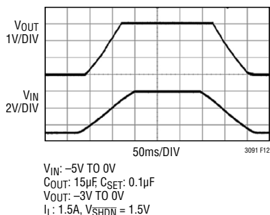
Figure 12. Floating Mode: Input Supply Ramp-Up and Down Using Positive \overline{SHDN} Bias Voltage
