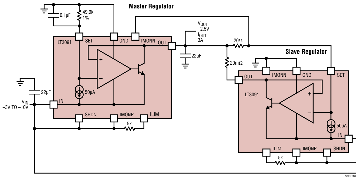
Paralleling Devices without Ballasting (50mA Minimum Load)
