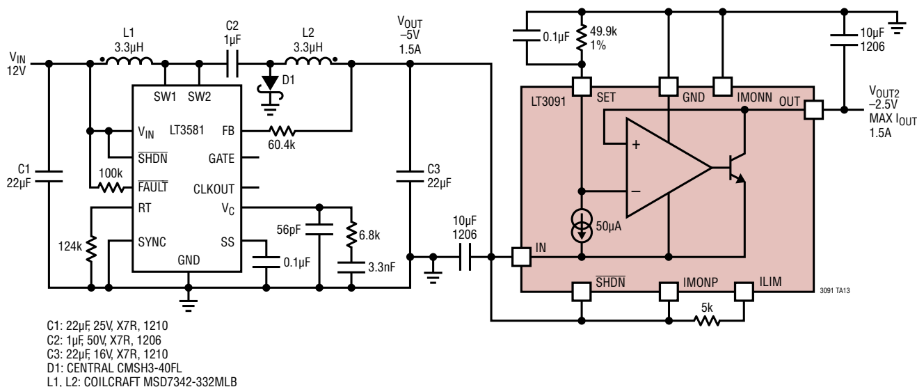
Low Noise Single Inductor Positive-to-Negative Converter
