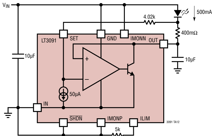
500mA LED Driver with Positive Supply
