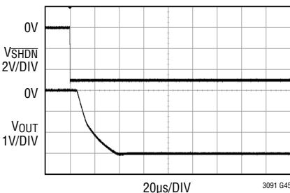
Fast \overline{\text{SHDN}} Start-Up
