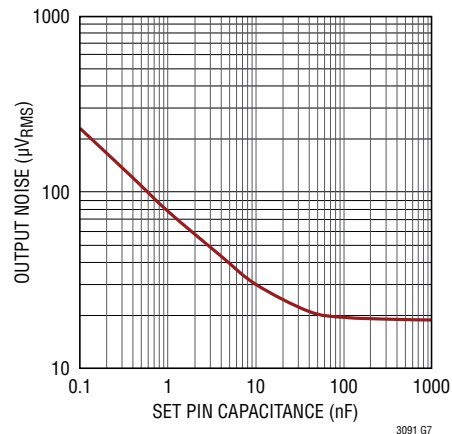
RMS Output Noise
