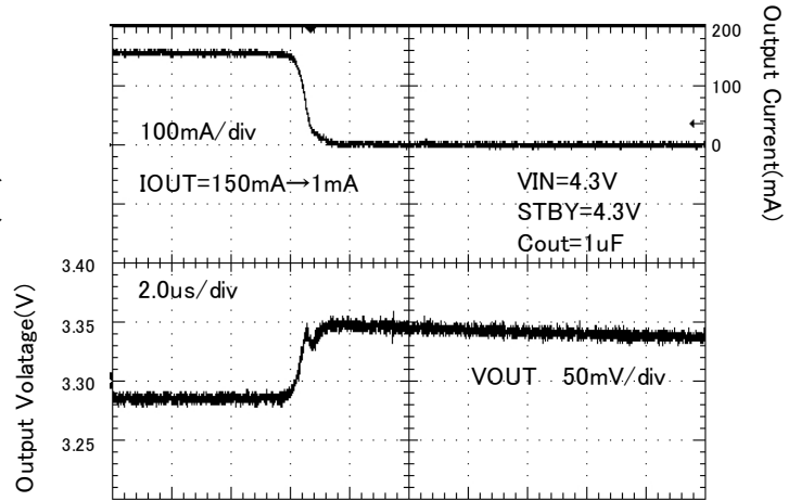
Figure 95. Load response (Iout = 150mA → 1mA)
