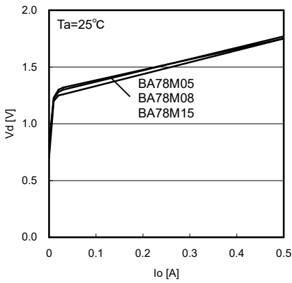
Fig.7 Dropout Voltage
