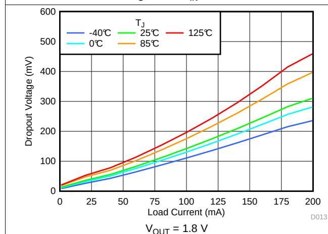
Figure 21. Dropout vs I_{OUT} and Temperature
