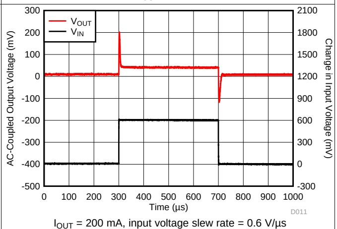
Figure 18. V_{IN} Transient
