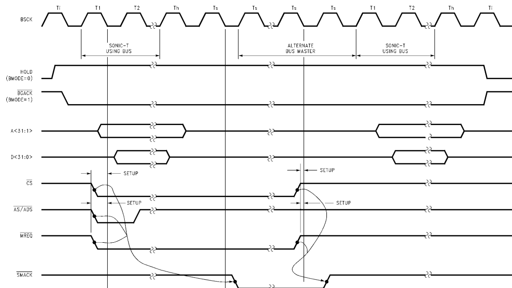
FIGURE 7-23. On-Chip Memory Arbitration
