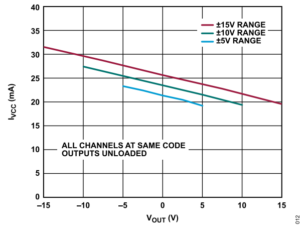
Figure 13. I_{ICC} vs. V_{OUT}
