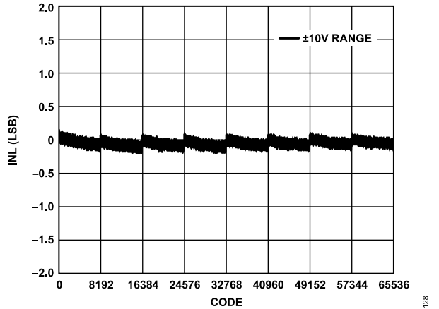
Figure 26. LTC2688-16 INL vs. Code
