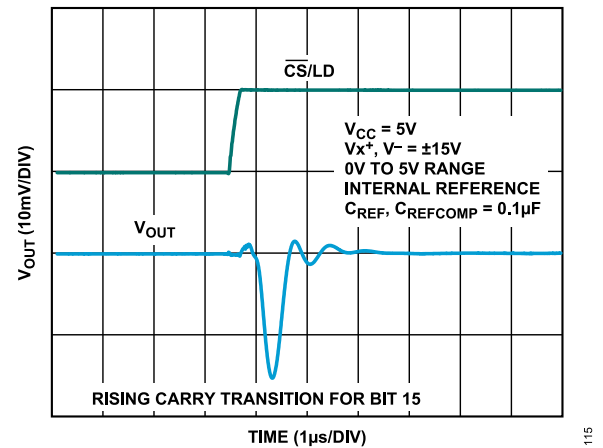
Figure 16. Glitch Impulse
