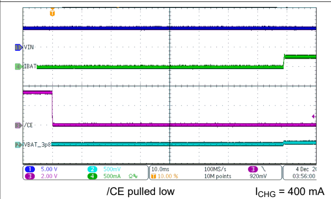
Figure 8-5. Charge Enable
