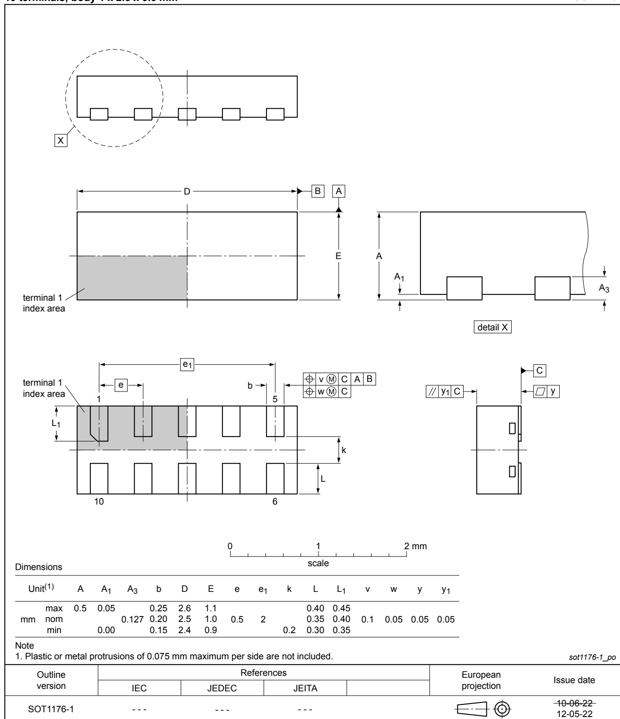
Fig. 15. Package outline DFN2510A-10 (SOT1176-1)
