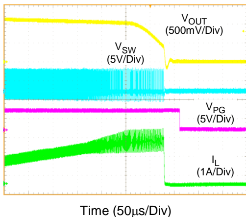
Figure 3. Over-Current Protection
