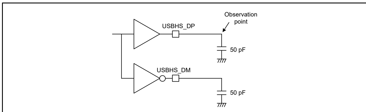
Figure 2.86 Test circuit in full-speed mode
