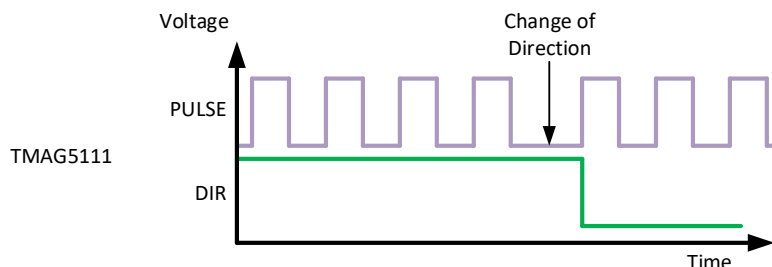
Figure 9-3. TMAG5111-Q1 Output Response
