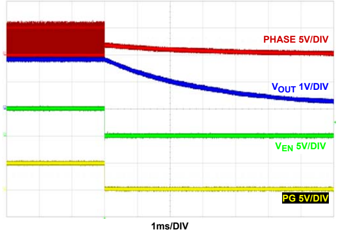
FIGURE 33. SHUTDOWN AT NO LOAD, V IN = 5V, MODE = PWM, T A = +25°C
