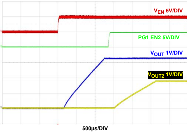
FIGURE 24. SEQUENTIAL START-UP USING EN AND PG AT FULL LOAD, V IN = 5V, MODE = PWM, T A = +25°C
