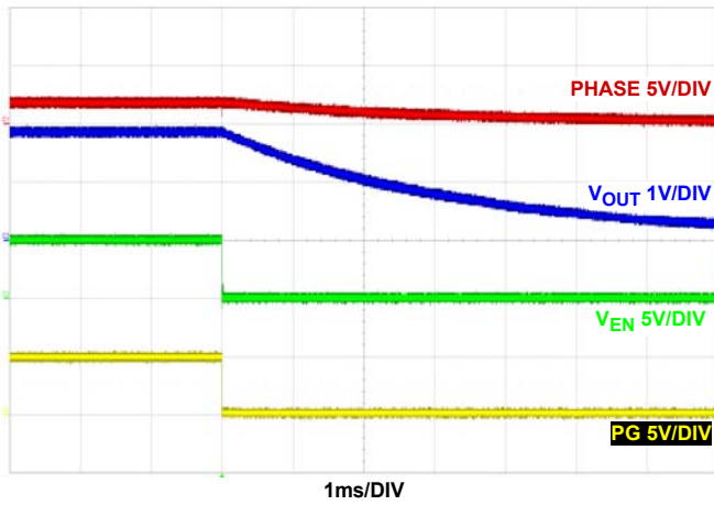
FIGURE 32. SHUTDOWN AT NO LOAD, V IN = 5V, MODE = PFM, T A = +25°C
