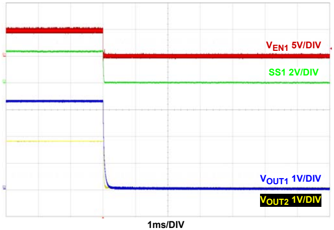
FIGURE 29. RATIOMETRIC SHUTDOWN WITH V OUT1 LEADING V OUT2 AT FULL LOAD, V IN = 5V, MODE = PWM, T A = +25°C
