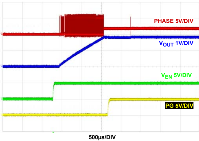
FIGURE 30. START-UP AT NO LOAD, V IN = 5V, MODE = PFM, T A = +25°C
