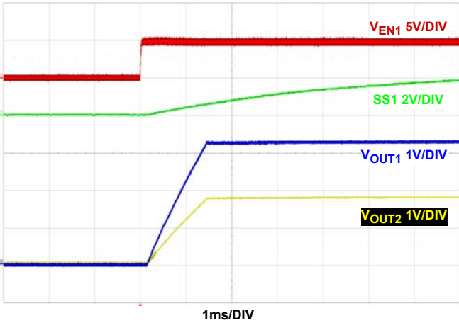
FIGURE 26. RATIOMETRIC START-UP WITH V OUT1 LEADING V OUT2 AT NO LOAD, V IN = 5V, MODE = PWM, T A = +25°C
