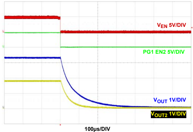
FIGURE 25. SEQUENTIAL SHUTDOWN USING EN AND PG AT FULL LOAD, V IN = 5V, MODE = PWM, T A = +25°C
