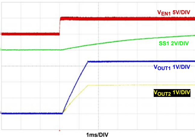
FIGURE 28. RATIOMETRIC START-UP WITH V OUT1 LEADING V OUT2 AT FULL LOAD, V IN = 5V, MODE = PWM, T A = +25°C
