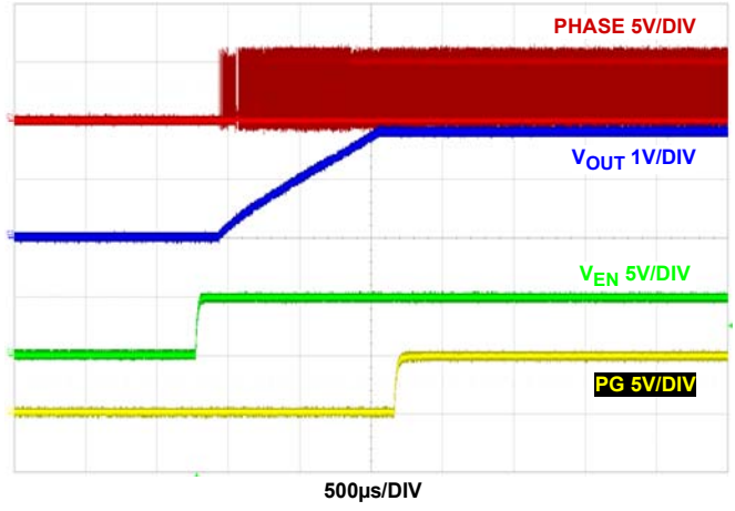
FIGURE 31. START-UP AT NO LOAD, V IN = 5V, MODE = PWM, T A = +25°C
