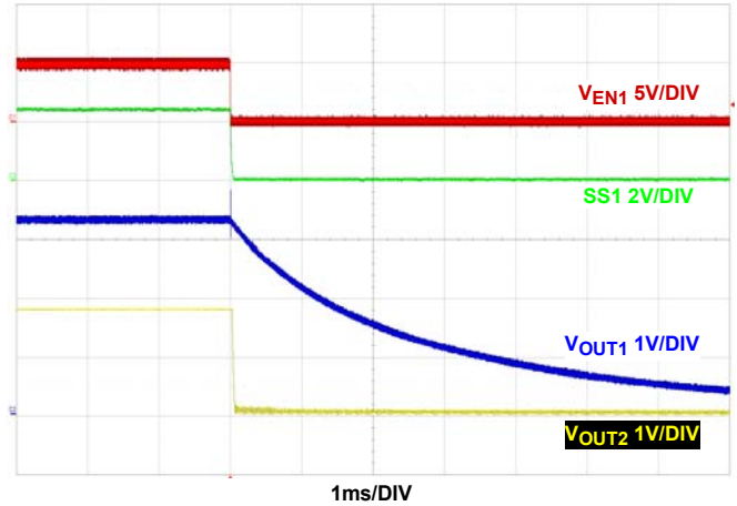
FIGURE 27. RATIOMETRIC SHUTDOWN WITH V OUT1 LEADING V OUT2 AT NO LOAD, V IN = 5V, MODE = PWM, T A = +25°C
