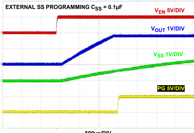
FIGURE 14. START-UP AT NO LOAD f_{SW} = 2\text{MHz} , V_{IN} = 5\text{V} , MODE = PWM, T_A = +25^\circ\text{C}
