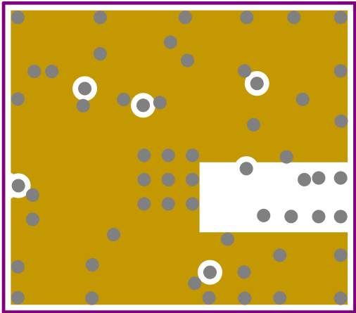
Figure 163: Mid layer 1
