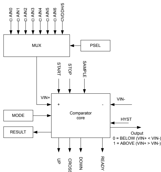
Figure 38: Comparator overview
