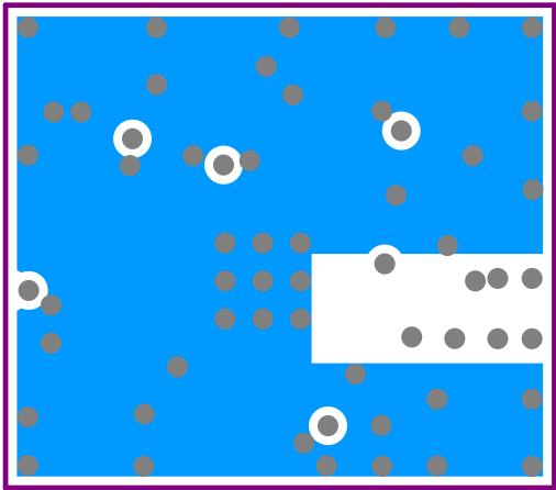
Figure 164: Mid layer 2
