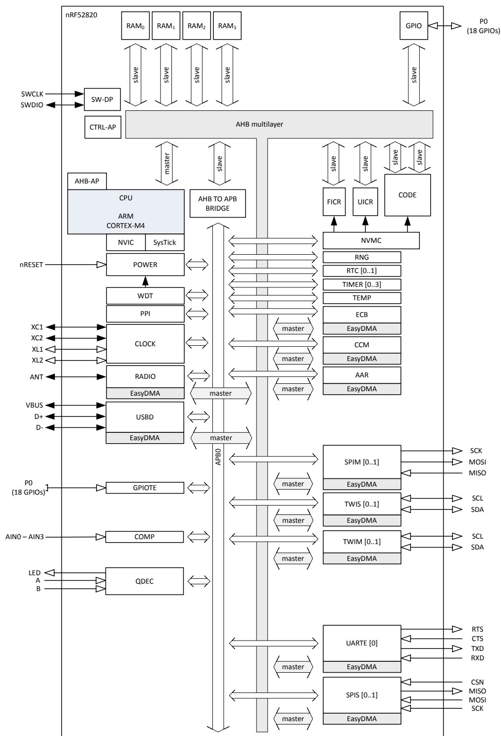
Figure 1: Block diagram
