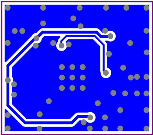
Figure 165: Bottom layer
