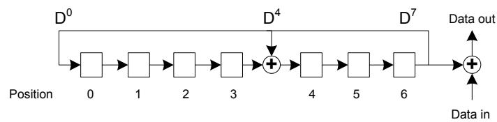
Figure 52: Data whitening and de-whitening
