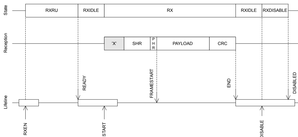
Figure 75: IEEE 802.15.4 receive sequence
