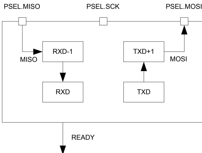
Figure 97: SPI master
