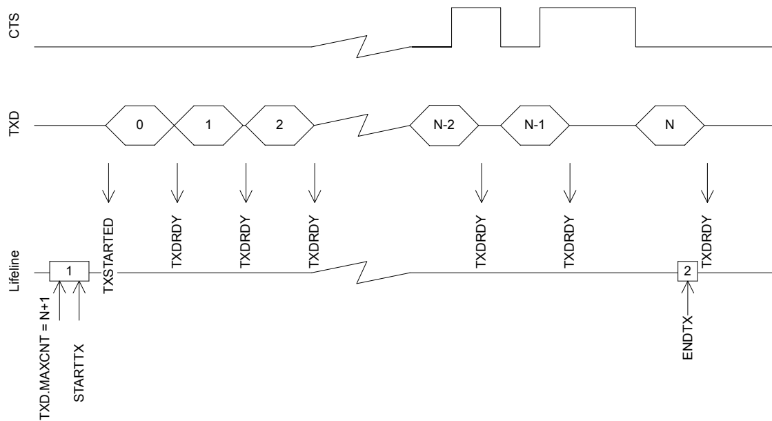
Figure 134: UART transmission
