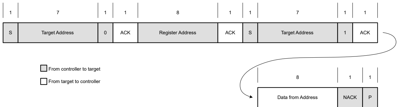
Figure 7-12. Single-Byte Read
